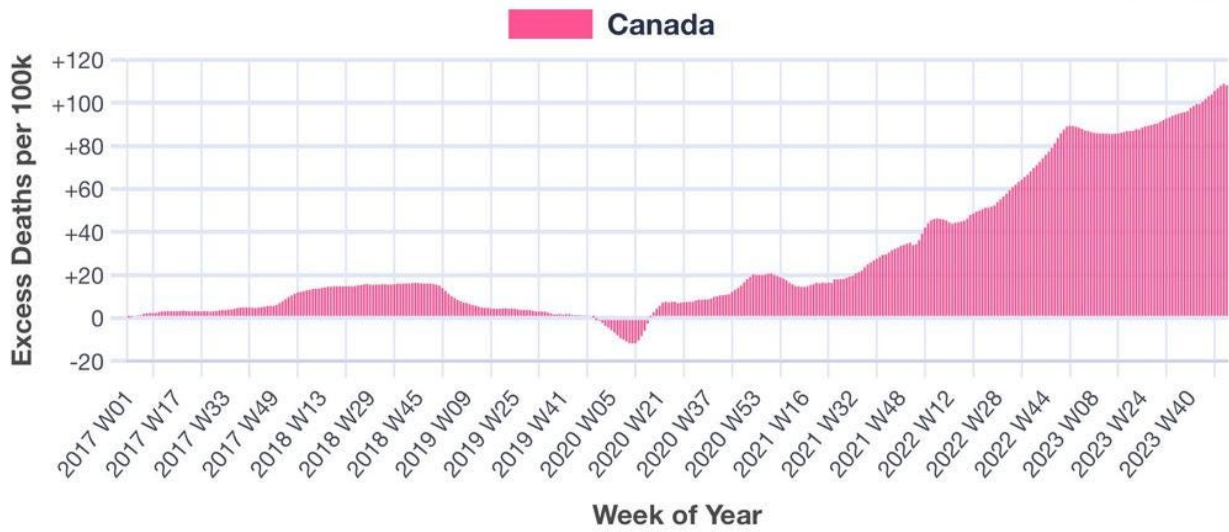
CAN 2020 Standard Population · Baseline: Average 2017 W01-2019 W52
