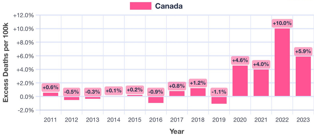
CAN 2020 Standard Population · Baseline: Linear Regression 2011-2019
