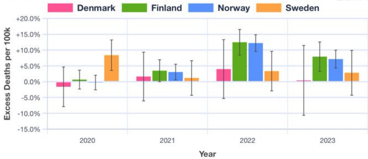
European Standard Population · Baseline: Linear Regression <2020 · 95% Prediction Interval
