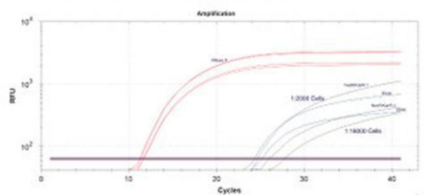
PCR detection of persistent Plasmid DNA
