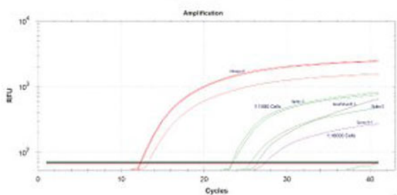
PCR detection of persistent Plasmid DNA
