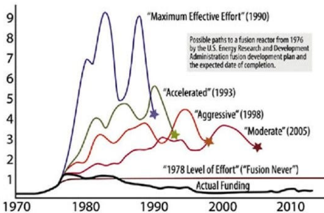
Credit: graphic design by Geoffrey M. Olynyk, incorporating 1976 projections from the U.S. Energy Research and Development Administration, "Fusion power by magnetic confinement: Program Plan," by S. O. Dean.
