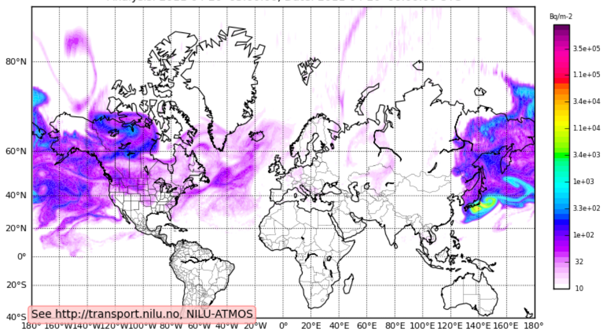
FUKUSHIMA Potential Releases: Xe-133, Total Column Analysis: 2011-04-20 03:00:00, Date: 2011-04-20 06:00:00 UTC
